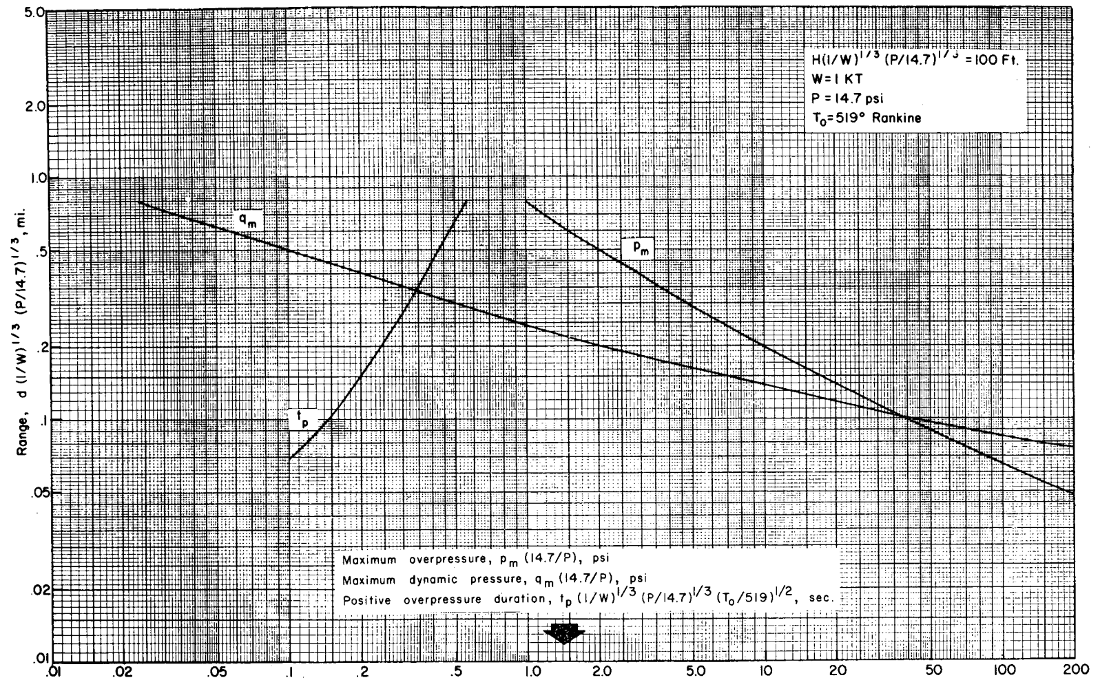
Fig. 2.2—Scaled blast parameters for a scaled height of burst of 100 ft as a function of scaled range. These are plots of Eqs. 2.18, 2.20, and 2.22 given in Table 2.2.
